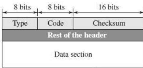
Error-reporting messages
